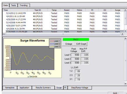
Baker AWA-IV screen with surge test results
