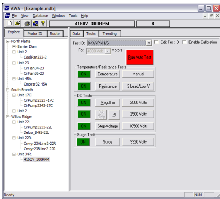
Baker AWA-IV test ID selection screen
